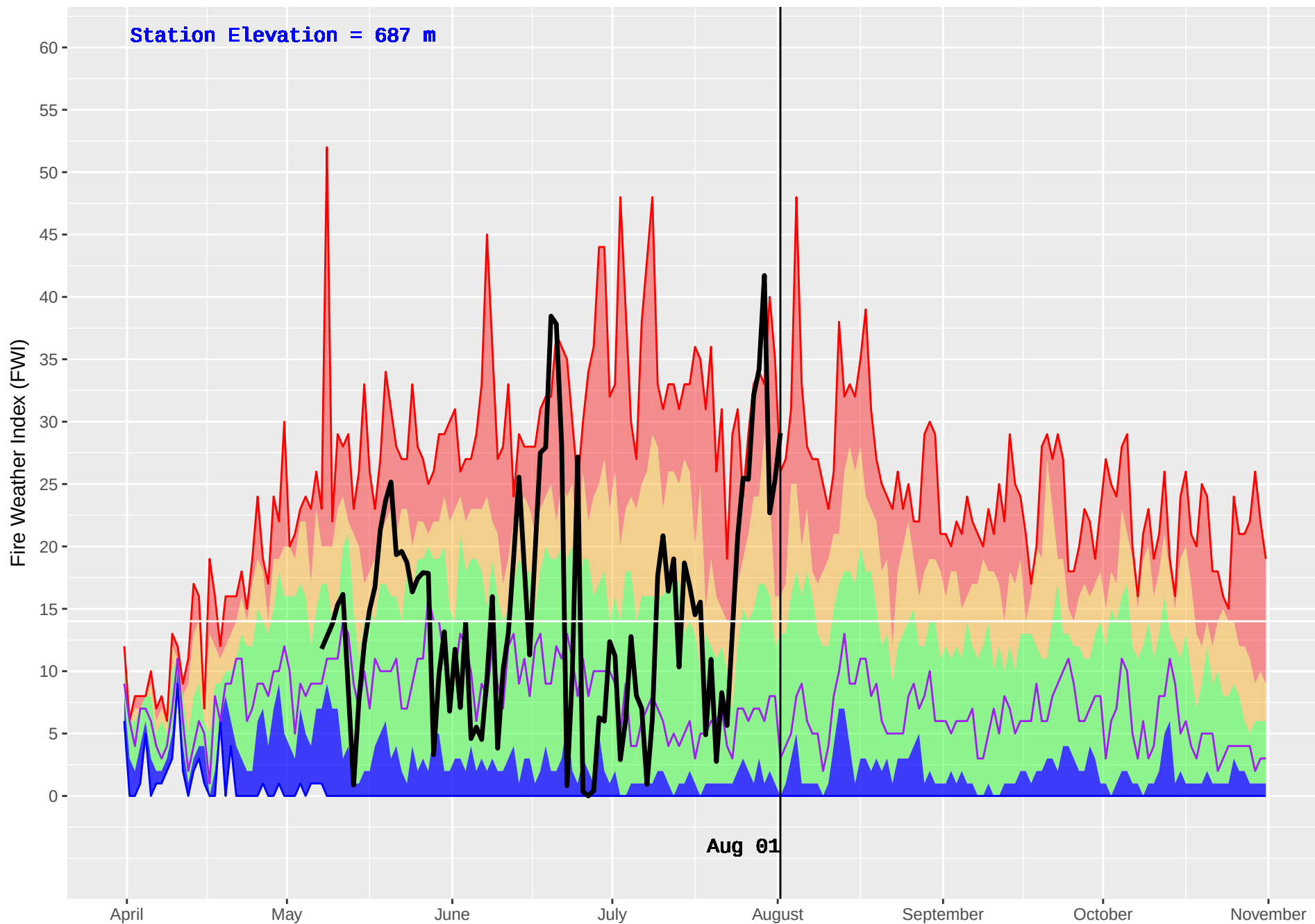
KETCHIKA (444) : Historical (1986–2016) and Current (2018) Daily Fire Weather Index (FWI)
