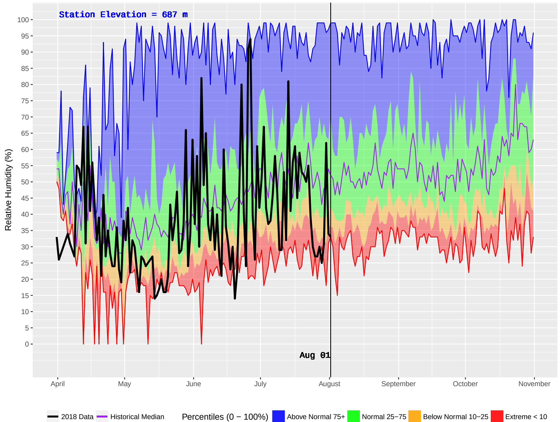
KETCHIKA (444) : Historical (1986–2016) and Current (2018) Daily Relative Humidity
